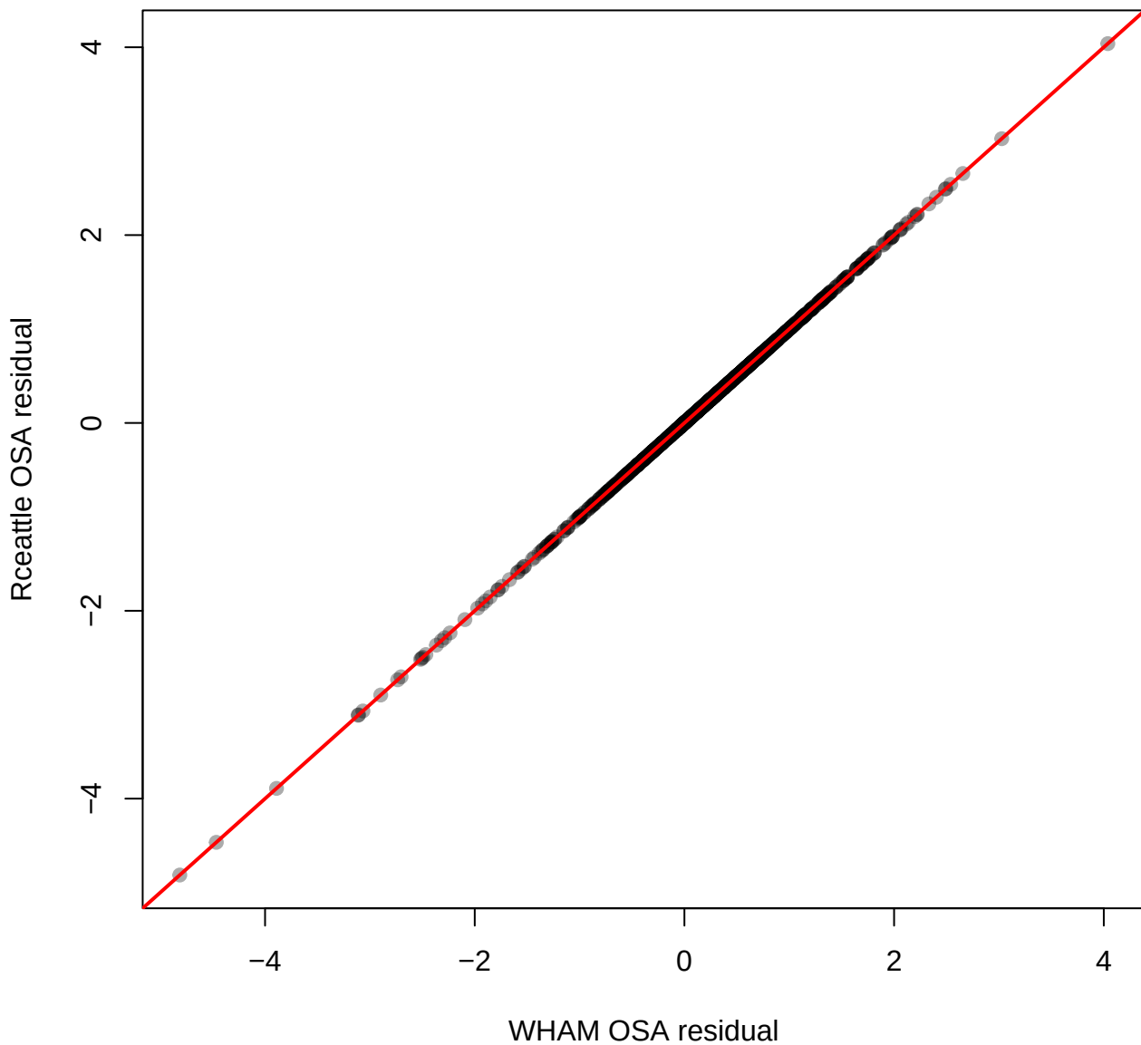
2021 GOA pollock OSA residuals (r = 1.000000)
